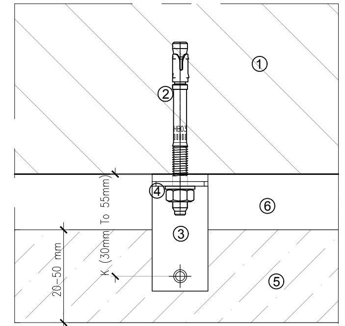
Horizontal Section Scale 1:2
