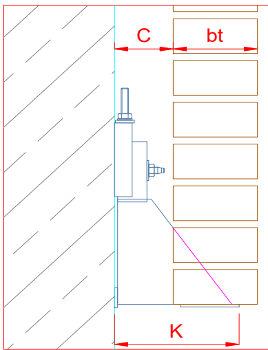
Wall Cavity and Projection
