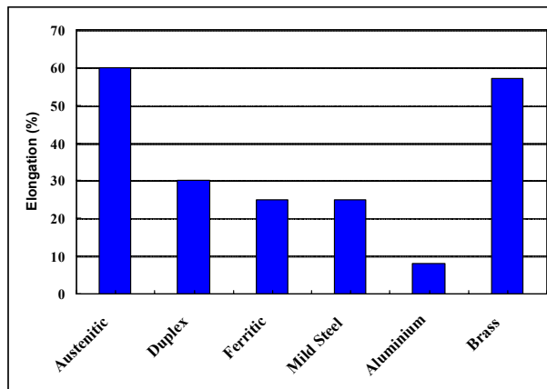
Figure 16 Typical elongations of annealed materials
