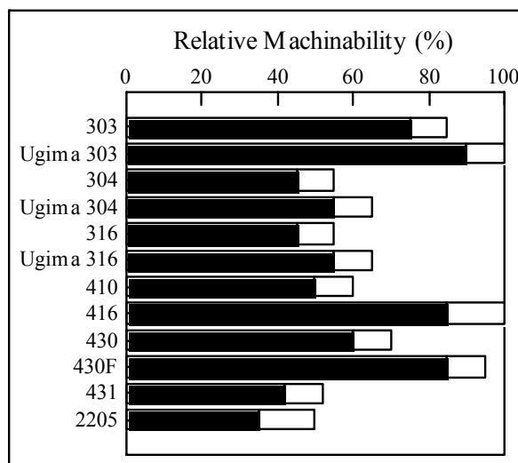
Figure 18 Relative machineabilities of stainless steels
