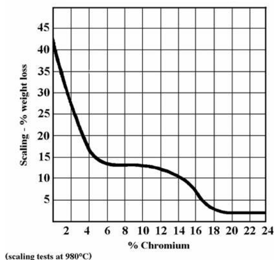
Figure 10 Effect of chromium content on scaling resistance
