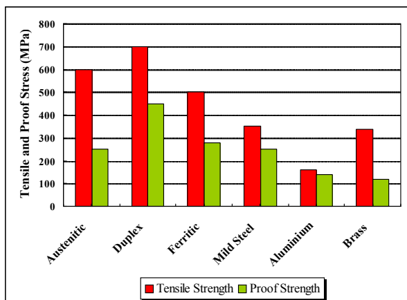
Figure 15 Typical tensile properties of annealed materials
