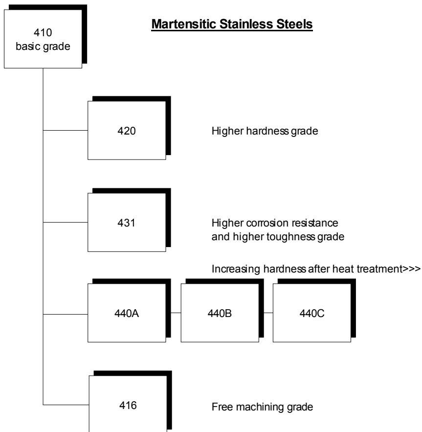
Figure 4 The families of Ferritic and Martensitic Stainless Steels
